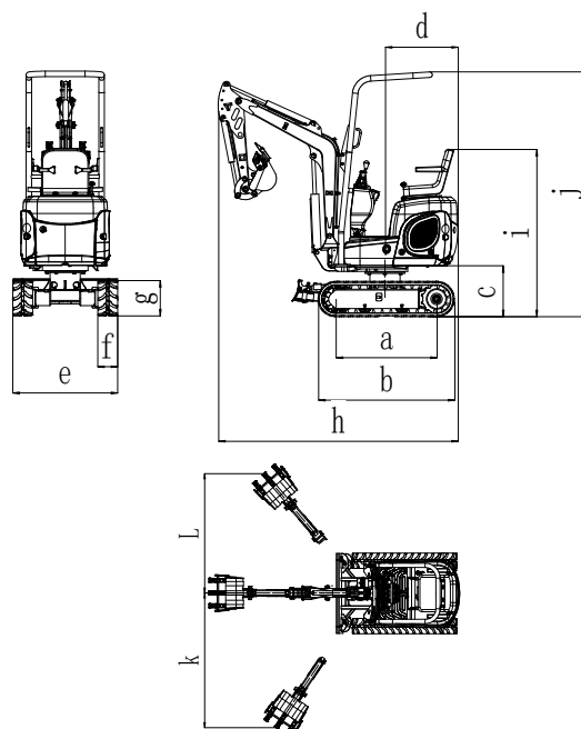
Main dimensions schematic diagram
